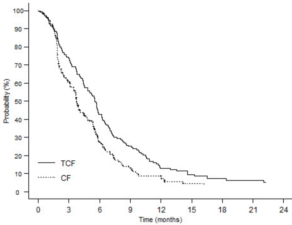
Figure 7: Gastric Cancer Study (TAX325) Survival K-M Curve
