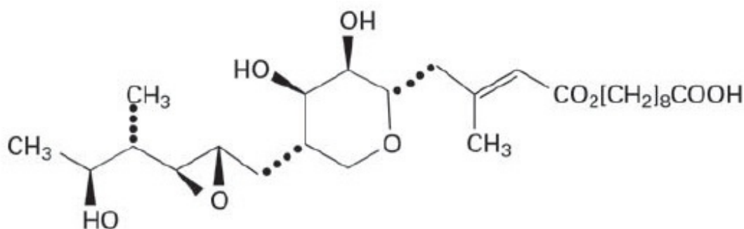
Figure 1. Structure of Mupirocin Figure 1. Structure of Mupirocin
