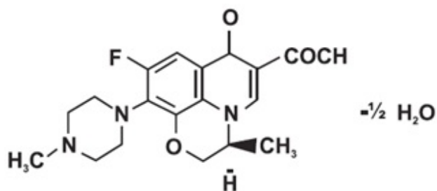
Figure 1: The Chemical Structure of Levofloxacin, USP
