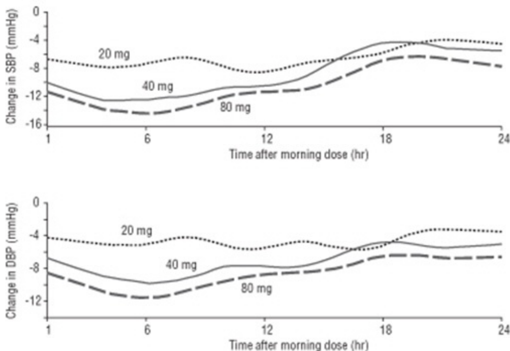
Figure 5. Changes from Baseline in Systolic Blood Pressure and Diastolic Blood Pressure Measured by 24-Hour ABPM
