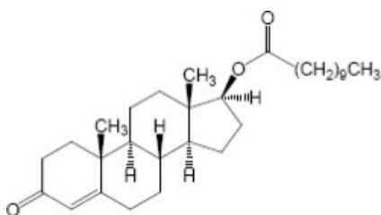
Figure 1: Testosterone Undecanoate
