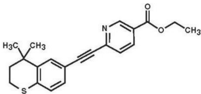
TAZAROTENE
