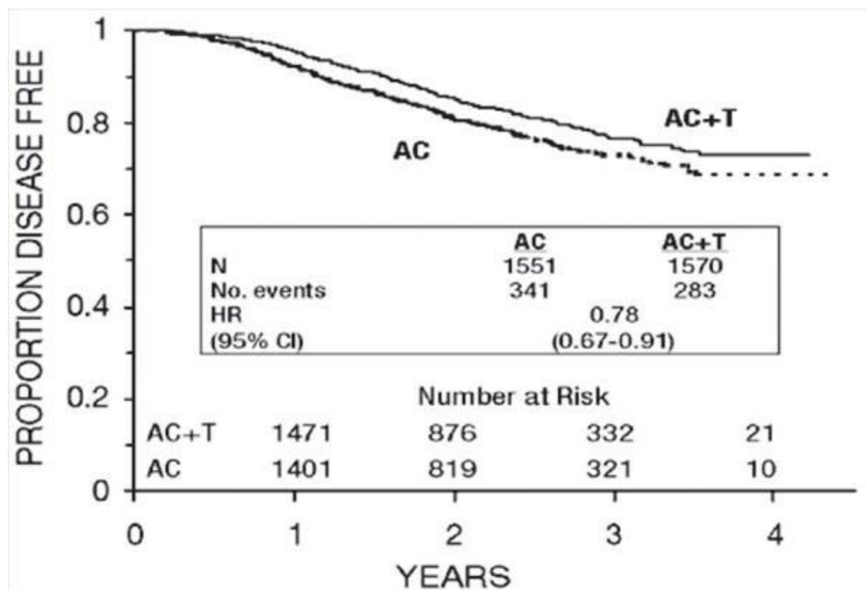
Figure 4. Survival: AC Versus AC+T
