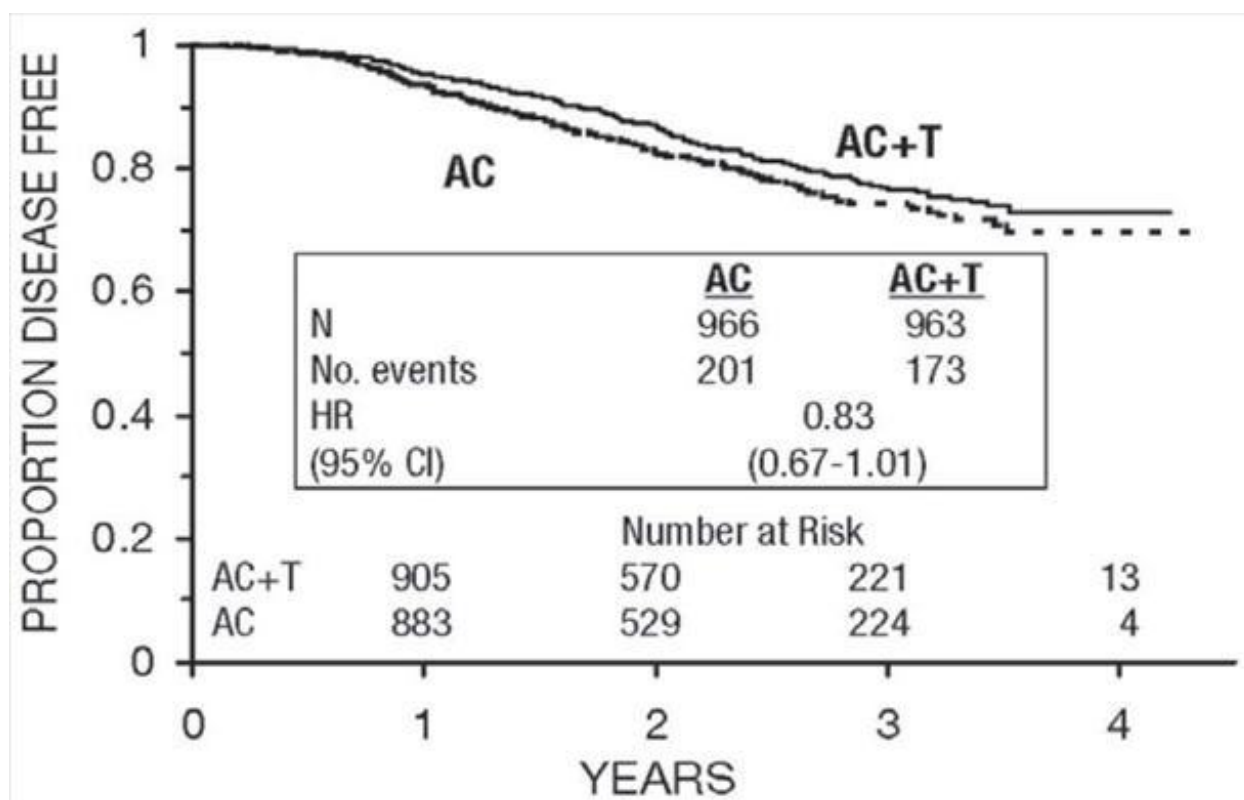
Figure 7. Disease-Free Survival: Premenopausal AC Versus AC+T
