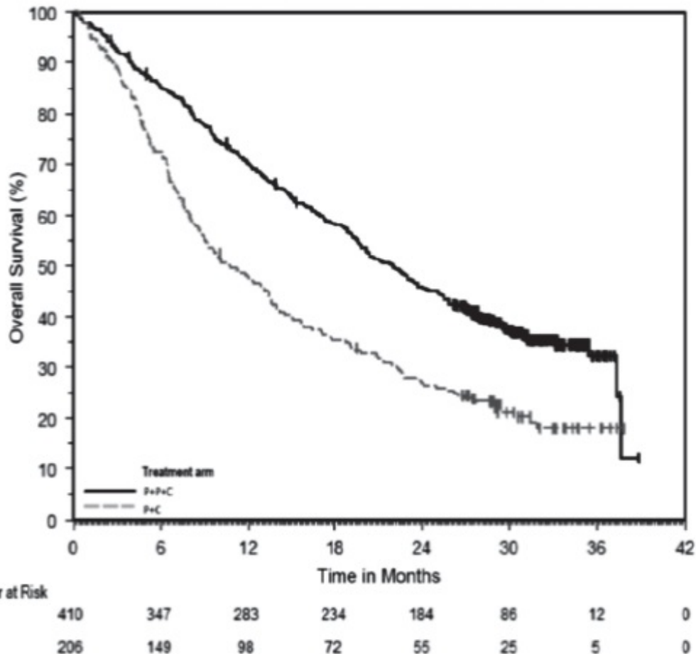
Figure 1: Kaplan-Meier Curve for Overall Survival in KEYNOTE-189
