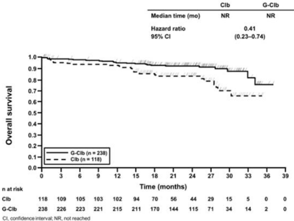
Figure 1 Kaplan-Meier Curve of Overall Survival in Patients with CLL in Study 1 (Stage 1)
