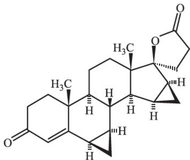
Drospirenone
