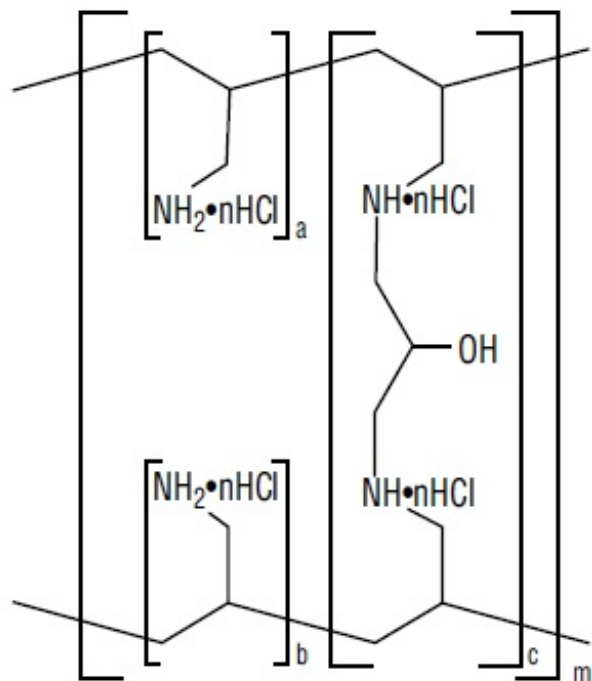
Figure 1: Chemical Structure of Sevelamer Hydrochloride
