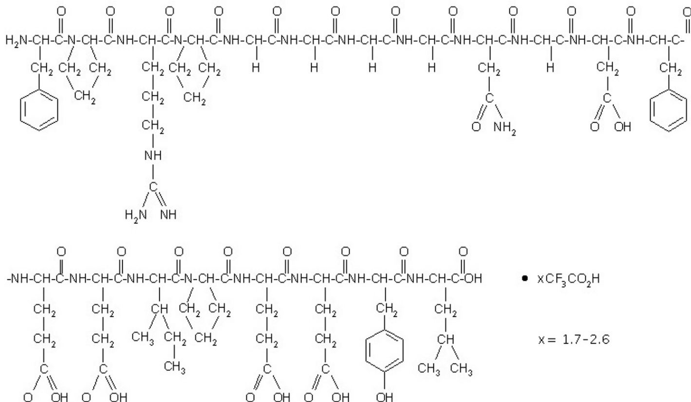
Figure 1: Structure Formula for Bivalirudin Trifluoroacetate
