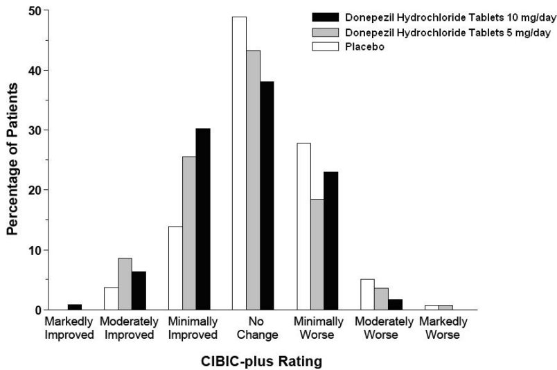
Figure 6. Frequency Distribution of CIBIC-plus Scores at Week 12.
