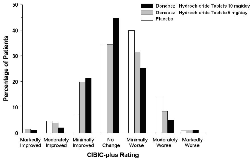
Figure 3. Frequency Distribution of CIBIC-plus Scores at Week 24.
