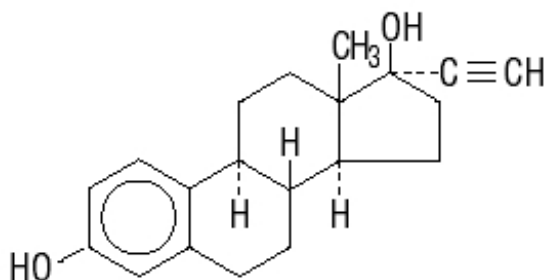
Ethinyl Estradiol, USP MW: 296.40 MF: C 20 H 24 O 2
