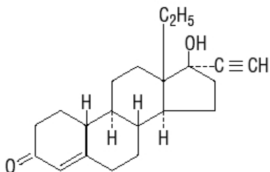
Levonorgestrel, USP MW: 312.45 MF: C 21 H 28 O 2
