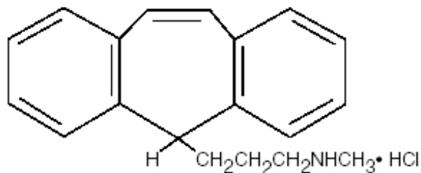
Figure 1 M.W. 299.84
