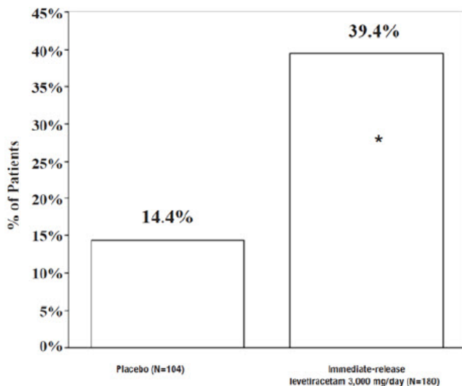
Figure 3: Responder Rate ( \geq 50\% Reduction From Baseline) In Study 4
