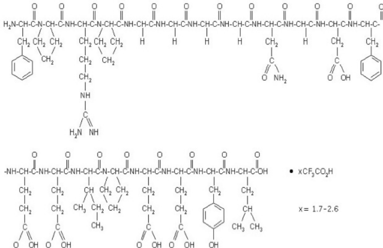
Figure 1. Structure formula for bivalirudin trifluoroacetate
