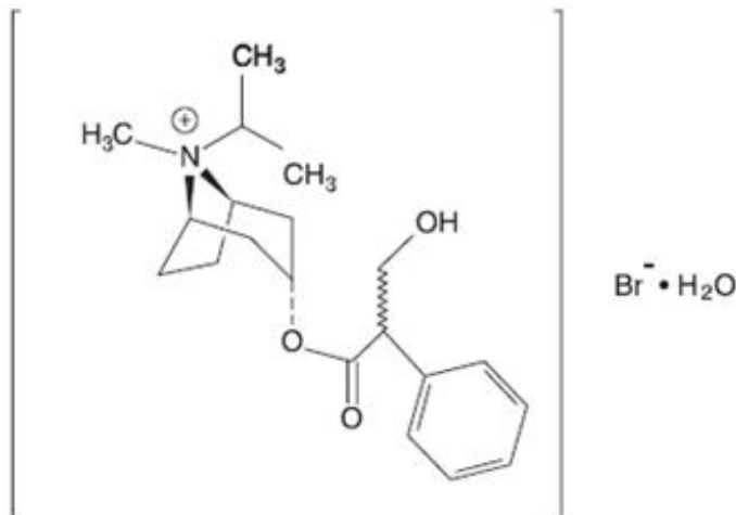
Figure 3.1-2. Chemical structure of ipratropium bromide.
