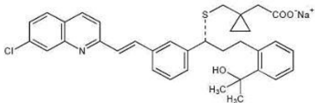
Chemical Structure
