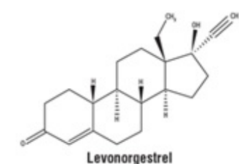
Figure 3. Structural Formulas
