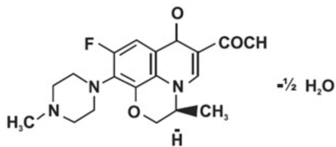
Figure 1: The Chemical Structure of Levofloxacin, USP
