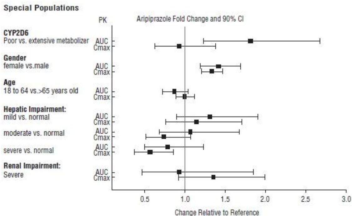
Figure 4: Effects of intrinsic factors on aripiprazole pharmacokinetics
