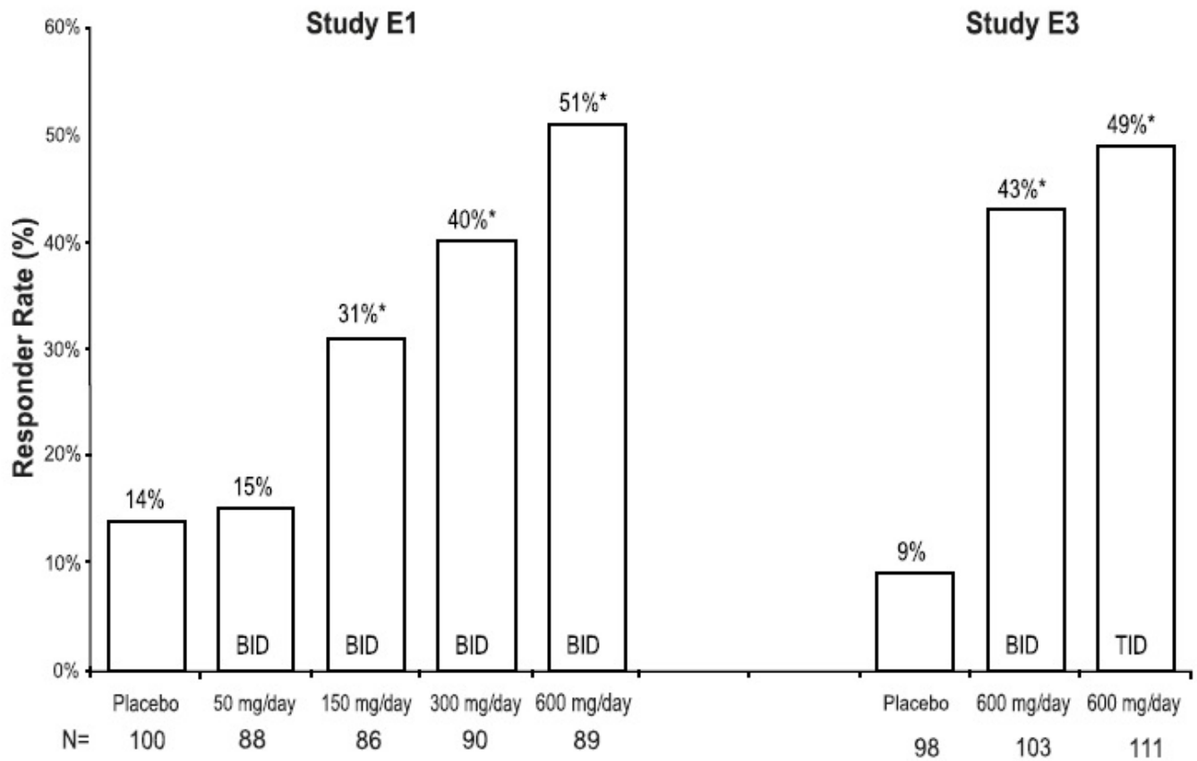
Figure 6: Responder Rate by Adjunctive Epilepsy Study
