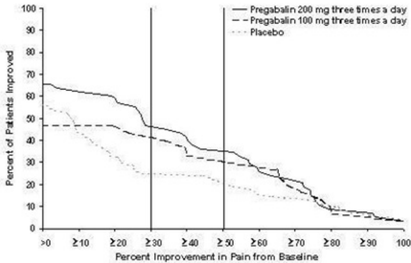
Figure 4: Patients Achieving Various Levels of Improvement in Pain Intensity – Study PHN
