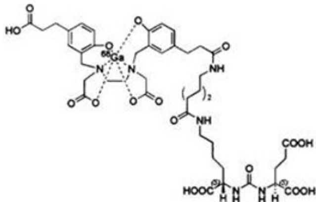
Figure 1: Chemical Structure of Gallium Ga Gozetotide
