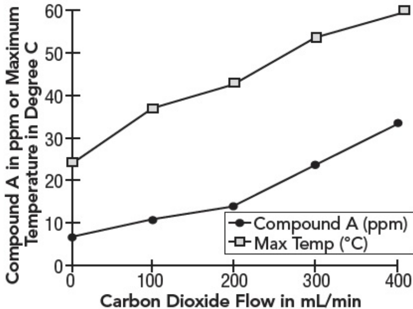
Figure 2. Carbon Dioxide Flow versus Compound A and Maximum Temperature
