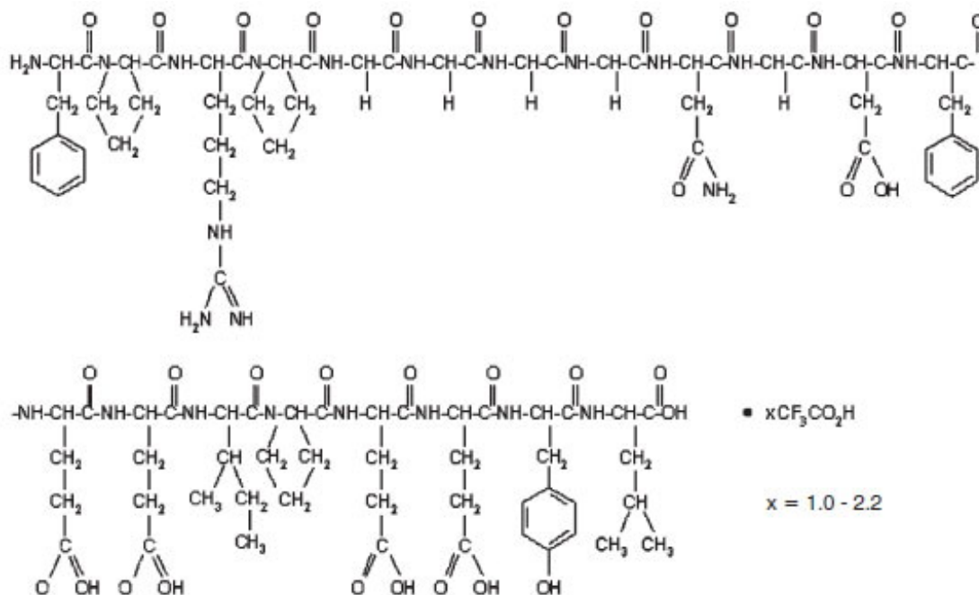
Figure 1. Structural formula for bivalirudin trifluoroacetate
