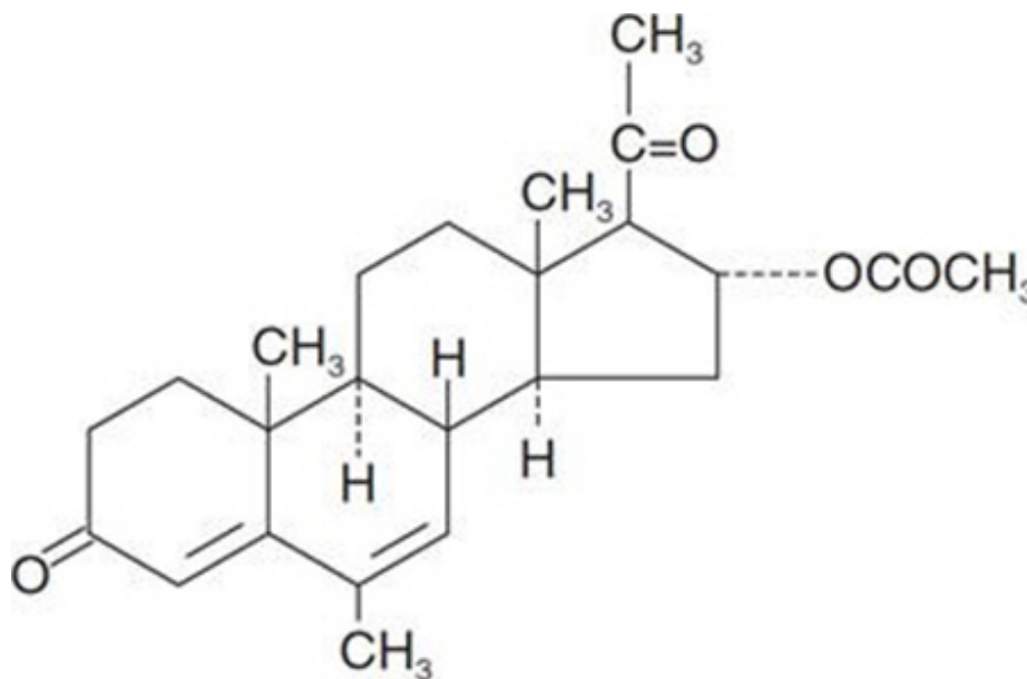
Figure 1: Megestrol Acetate Chemical Structure
