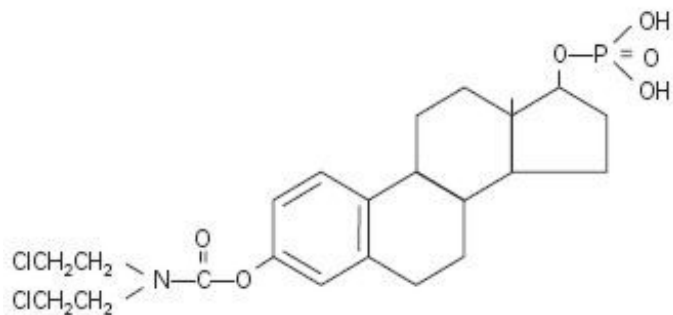
Figure 1. Estramustine Phosphate
