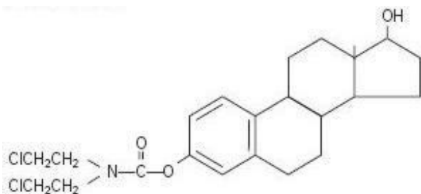
Figure 2. Estramustine
