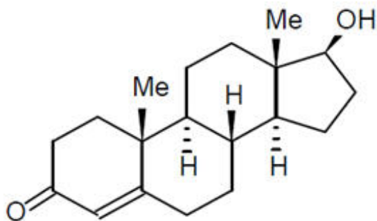
Testosterone (C 19 H 28 O 2 )
