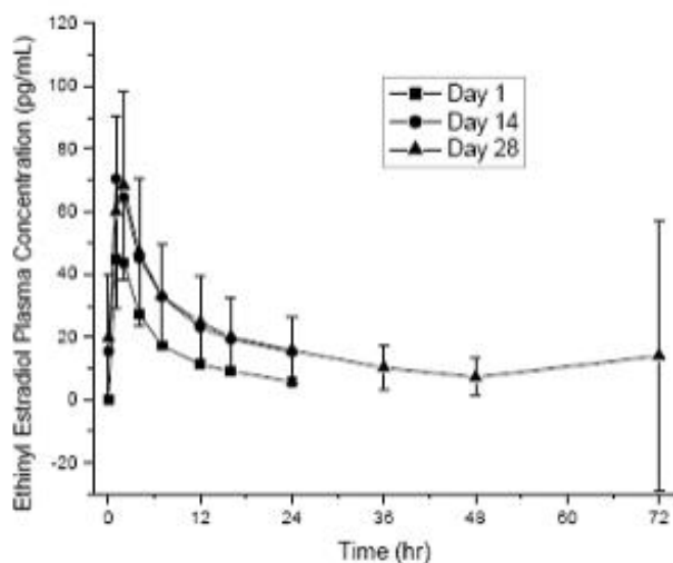
Figure 1: Mean Plasma \pm SD † Concentrations of Levonorgestrel and Ethinyl Estradiol Following Single (Day 1) and Multiple (Days 14 and 28) Oral Administrations of Levonorgestrel 90 mcg in Combination with Ethinyl Estradiol 20 mcg to Healthy Women
