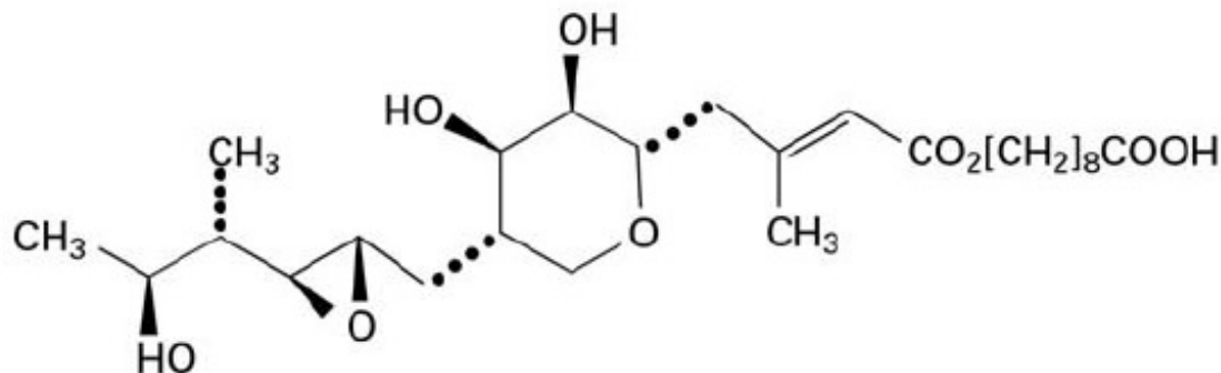
Figure 1. Structure of Mupirocin
