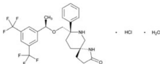
rolapitant hydrochloride
