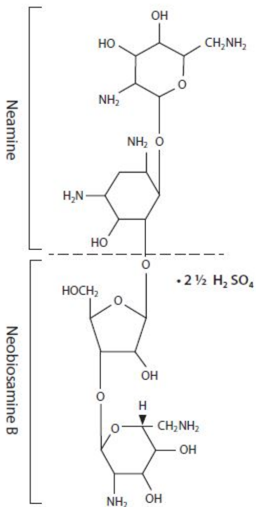
Neomycin B Sulfate C_{23}H_{46}N_6O_{13} \cdot 2\frac{1}{2}H_2SO_4 MW 614.67
