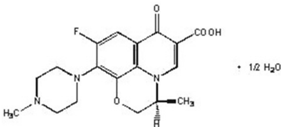
Figure 1: The Chemical Structure of Levofloxacin
