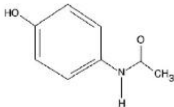
Acetaminophen C_8H_9NO_2 MW = 151.16
