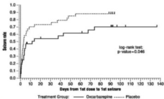
Figure 2: Kaplan-Meier Estimates of First Seizure Event Rate by Treatment Group
