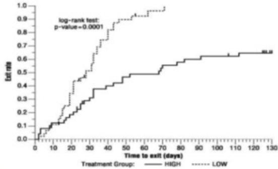
Figure 3: Kaplan-Meier Estimates of Exit Rate by Treatment Group
