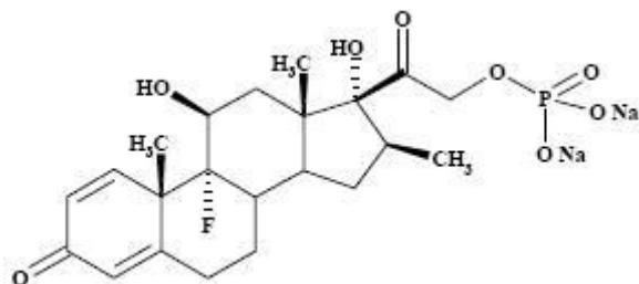
Structural Formula
