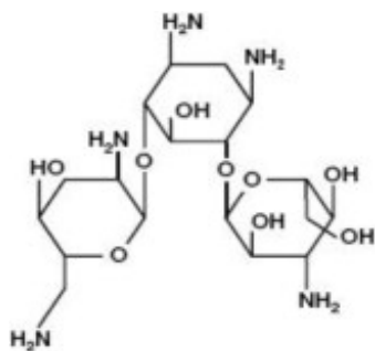
Figure 2: Tobramycin Structure
