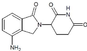
3-(4-amino-1-oxo-1,3-dihydro-2H-isindol-2-yl) piperidine-2,6-dione
