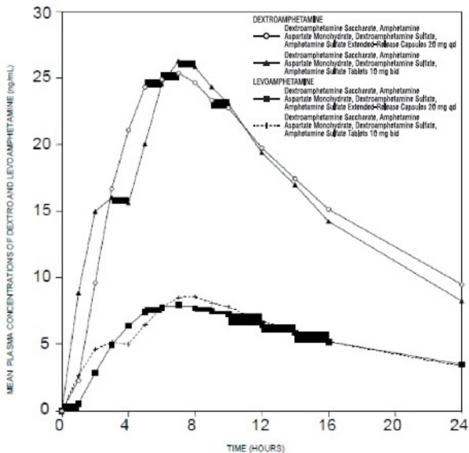
Figure 1 Mean d-amphetamine and l-amphetamine Plasma Concentrations Following Administration of Dextroamphetamine Saccharate, Amphetamine Aspartate Monohydrate, Dextroamphetamine Sulfate, Amphetamine Sulfate Extended-Release Capsules 20 Mg (8 Am) And Dextroamphetamine Saccharate, Amphetamine Aspartate Monohydrate, Dextroamphetamine Sulfate, Amphetamine Sulfate Tablets (Immediate-Release) 10 mg Twice Daily (8 am and 12 noon) in the Fed State.
