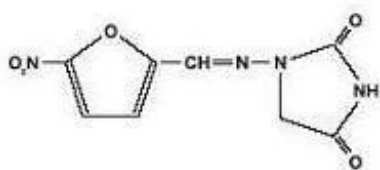
1-[[[(5-nitro-2-furanyl)methylene]amino]-2, 4-imidazolidinedione
