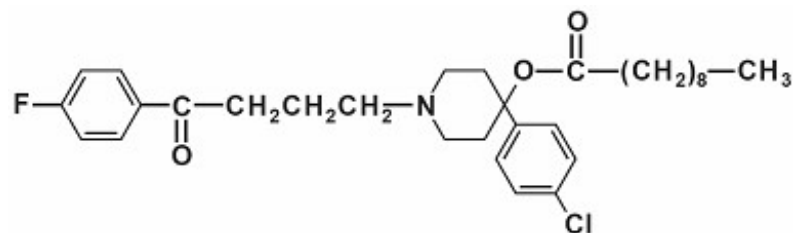
Structural Formula
