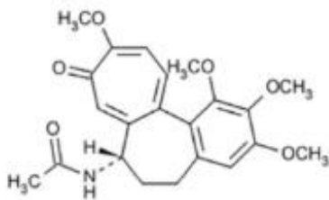
Figure 1: Colchicine Structural Formula
