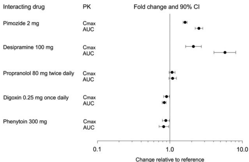
Figure 1. Impact of Paroxetine on the Pharmacokinetics of Co-Administered Drugs (log
