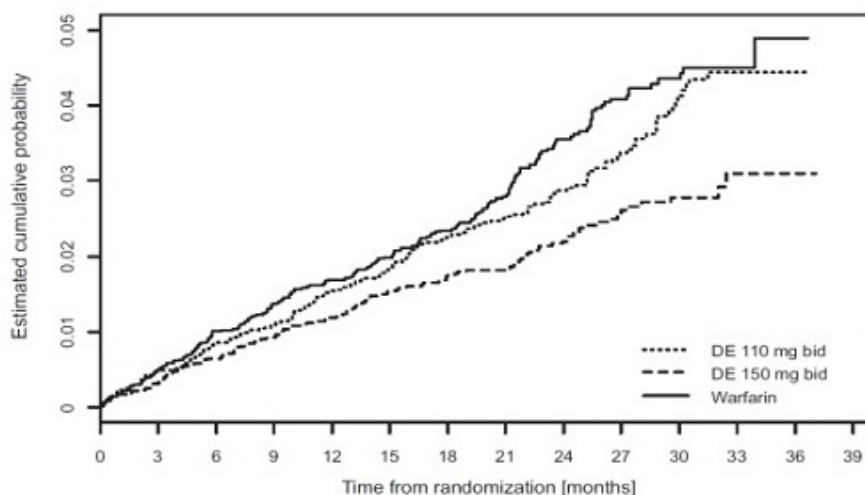
Figure 4: Kaplan-Meier Curve Estimate of Time to First Stroke or Systemic Embolism
