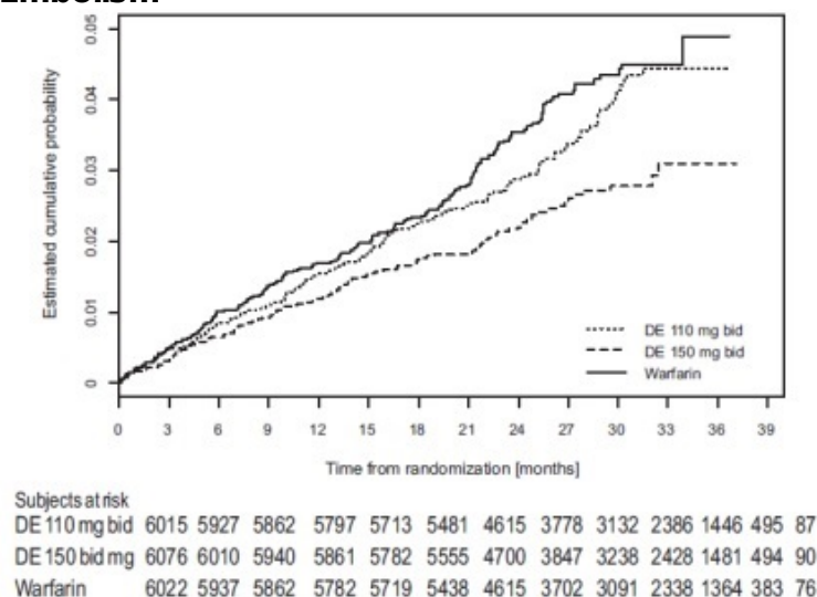
Figure 4: Kaplan-Meier Curve Estimate of Time to First Stroke or Systemic Embolism
