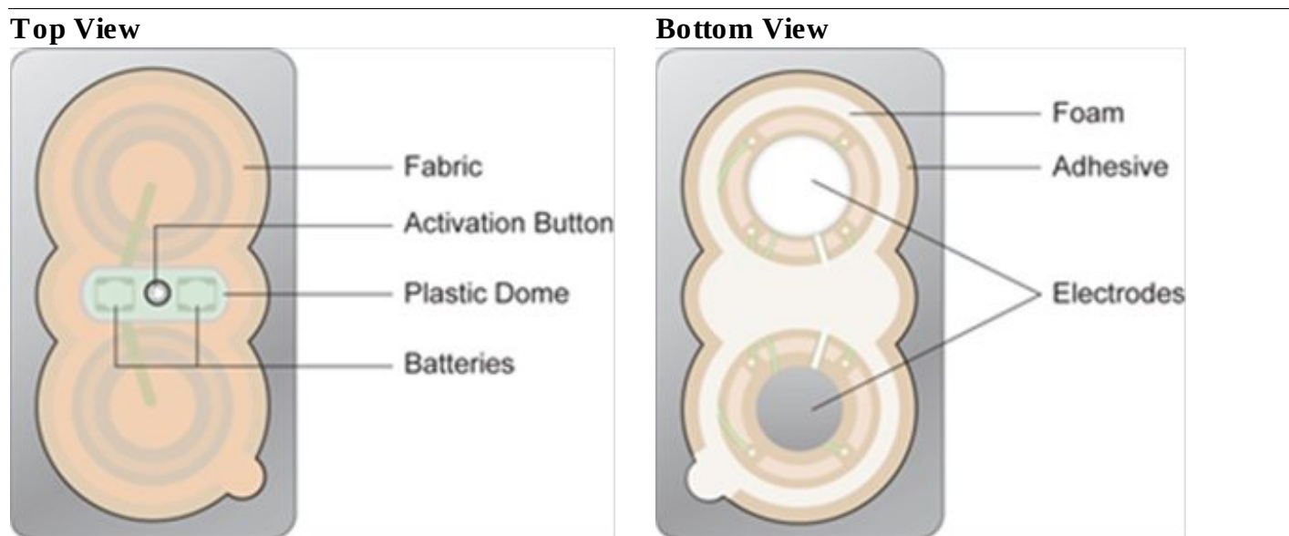
Figure 2: Iontophoretic Device
