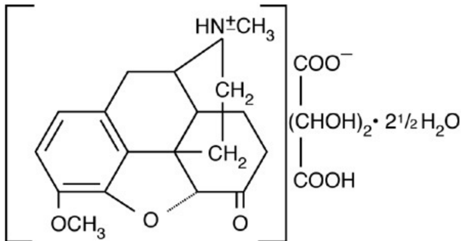
Hydrocodone Bitartrate Structural Formula
