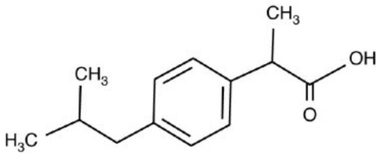
Ibuprofen Structural Formula
