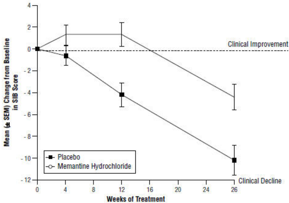
Figure 3: Time course of the change from baseline in SIB score for patients completing 28 weeks of treatment.
