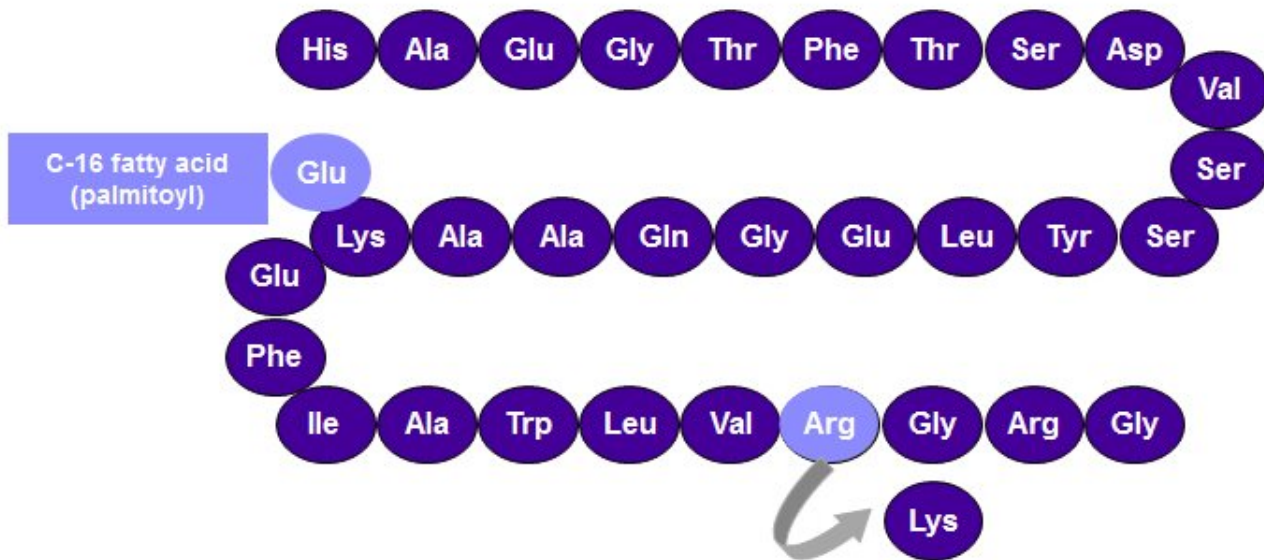
Figure 1. Structural Formula of liraglutide
