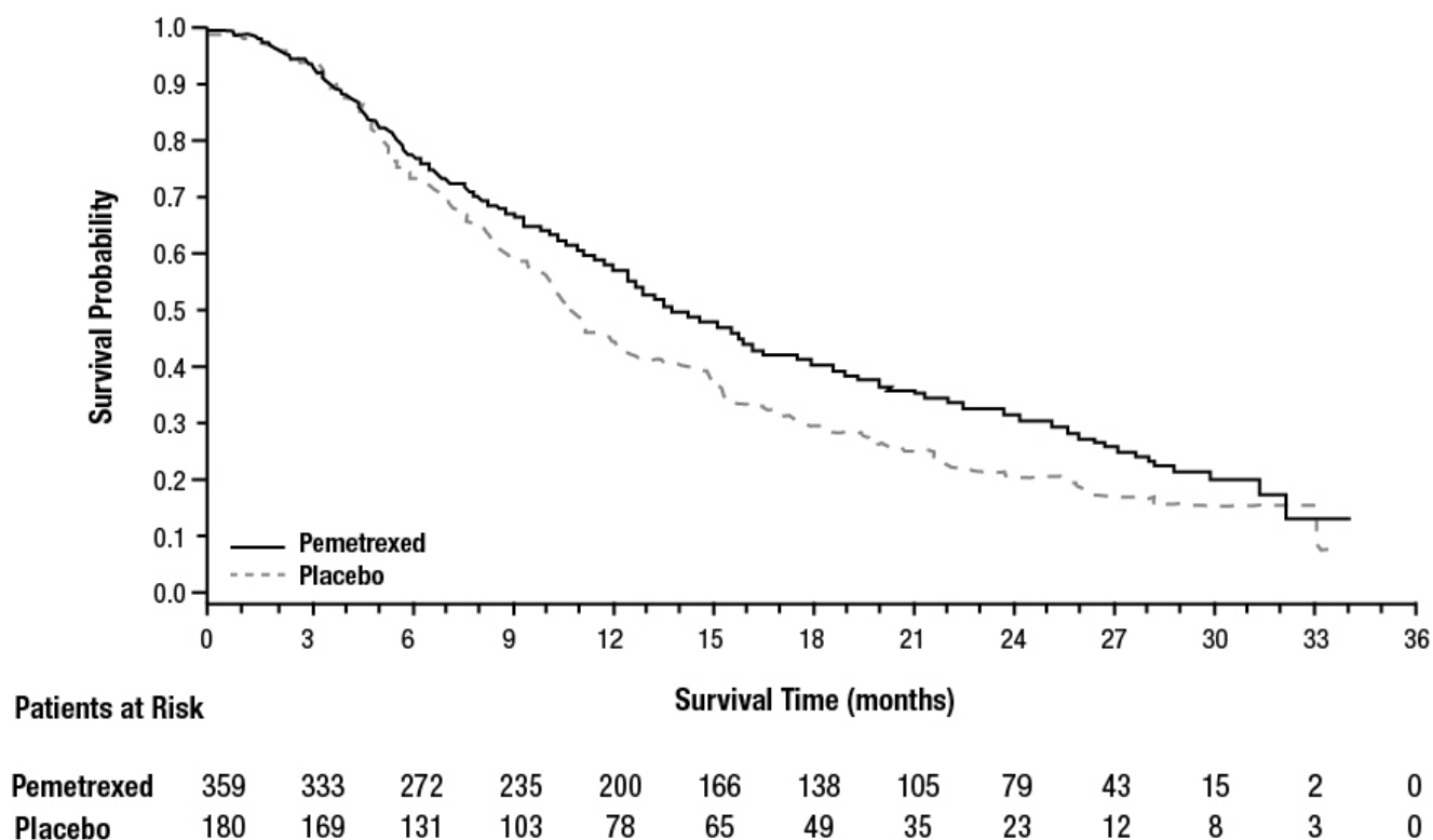
Figure 8: Kaplan-Meier Curves for Overall Survival in PARAMOUNT
